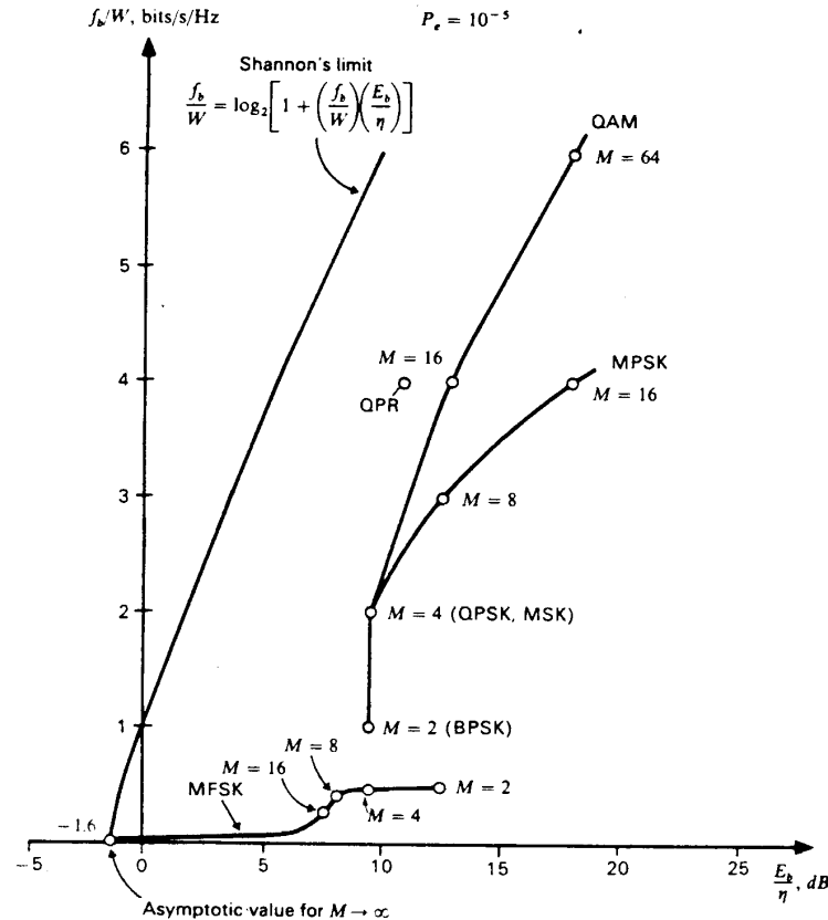
bits/s/Hz vs. E_b/\eta for Probability of Error = 10^{-5} taken from "Principle of Communication Systems" Taub & Schilling, page 482
