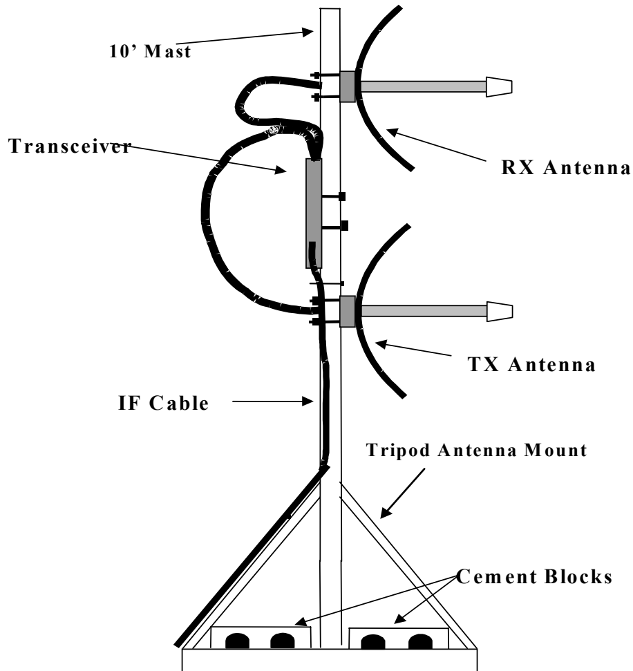
Non-penetrating Roof Mount Configuration
